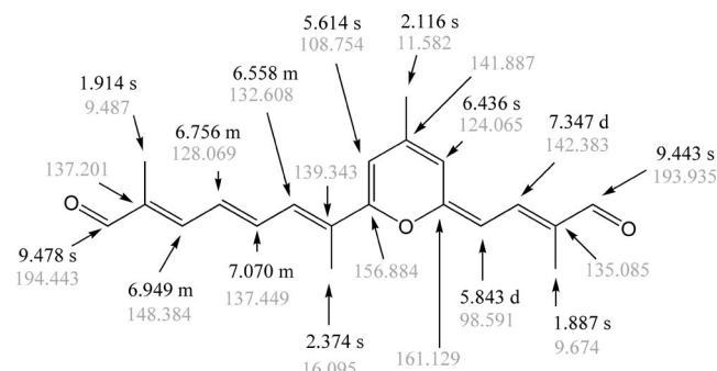
Scheme 7. Structure and ^1\text{H} and ^{13}\text{C} NMR data for \text{C}_{20} -pyran carotenoid 2 .
